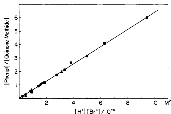
Figure 1. Product ratios against [H^+][Br^-] for equilibria established at 25 °C in 50:50 (v/v) trifluoroethanol/water ( I = 0.50 , NaClO 4 ): (●), [Br^-] = 0.022 M and [H^+] = 1 \times 10^{-4} to 1.7 \times 10^{-3} M; (■), [Br^-] = 0.044 M and [H^+] = 1 \times 10^{-4} to 7 \times 10^{-4} M; (▲), [Br^-] = 0.089 M and [H^+] = 1 \times 10^{-4} to 7 \times 10^{-4} M; (●), [Br^-] = 0.1334 M and [H^+] = 1 \times 10^{-4} to 7 \times 10^{-4} M.
