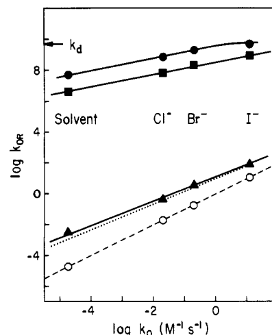
Figure 4. Logarithmic plot of the rate constants, k_o , for the reaction of solvent and halide ions with 1 against the following: ( \blacktriangle ) rate constants for the hydrogen ion catalyzed addition of nucleophiles to 1 , dotted line shows the correlation using data for halide ions only; ( \blacksquare ) rate constants for the addition of nucleophiles to 4-MeOArC(CF 3 ) 2 + ; ( \bullet ) rate constants for the addition of nucleophiles to 4-MeOArCH(CF 3 ) + ; ( \circ ) rate constants k_o for the addition of nucleophiles to 1 , dashed line shows the slope expected for an electrophile with the same nucleophile selectivity as 1 . The rate constants have the following units: \text{s}^{-1} ( \bullet , \blacksquare , \circ ) or \text{M}^{-1} \text{s}^{-1} ( \blacktriangle ) for the addition of solvent and \text{M}^{-1} \text{s}^{-1} ( \bullet , \blacksquare , \circ ) or \text{M}^{-2} \text{s}^{-1} ( \blacktriangle ) for the addition of halide ions. The estimated rate constant for a diffusion-limited reaction, k_d = 5 \times 10^9 \text{ M}^{-1} \text{ s}^{-1} , is also labeled.
